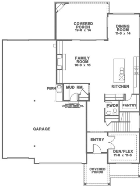
MAIN FLOOR
