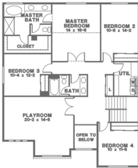
UPPER FLOOR
